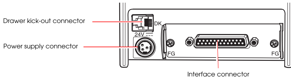
Figure 1-2 Connector panel
