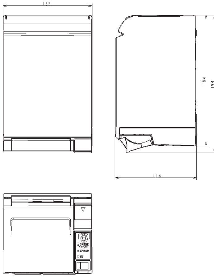
Figure 5-25 Dimensions
